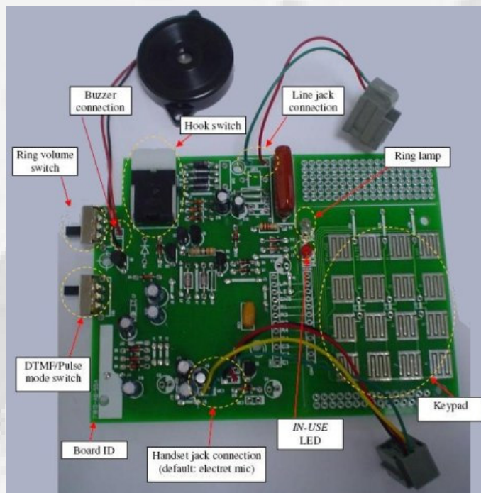
Figure 1.1: Demo board upper view
