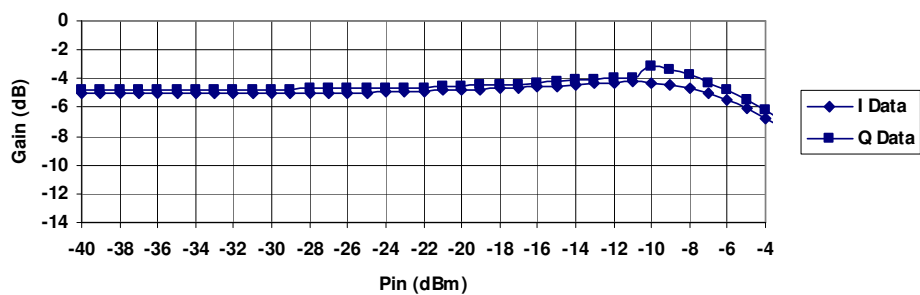
Gain VS Pin, Low Gain Mode
